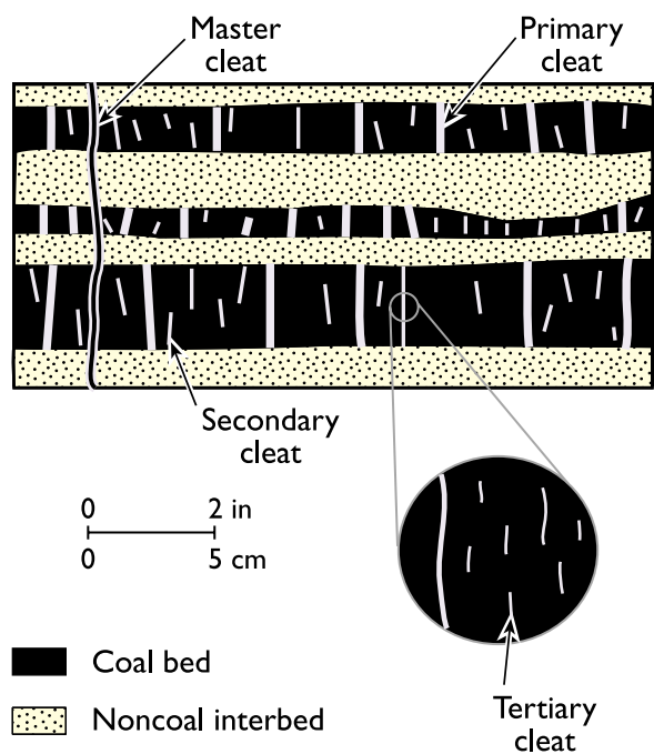
FIGURE 5 Diagram of vertical slice through coal reservoirs, showing vertical distribution of cleats (fractures) in the coal. From New Mexico Bureau of Geology and Mineral Resources, Bulletin 146.
